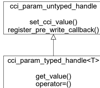
Figure 4 - cci_param_handle hierarchy
