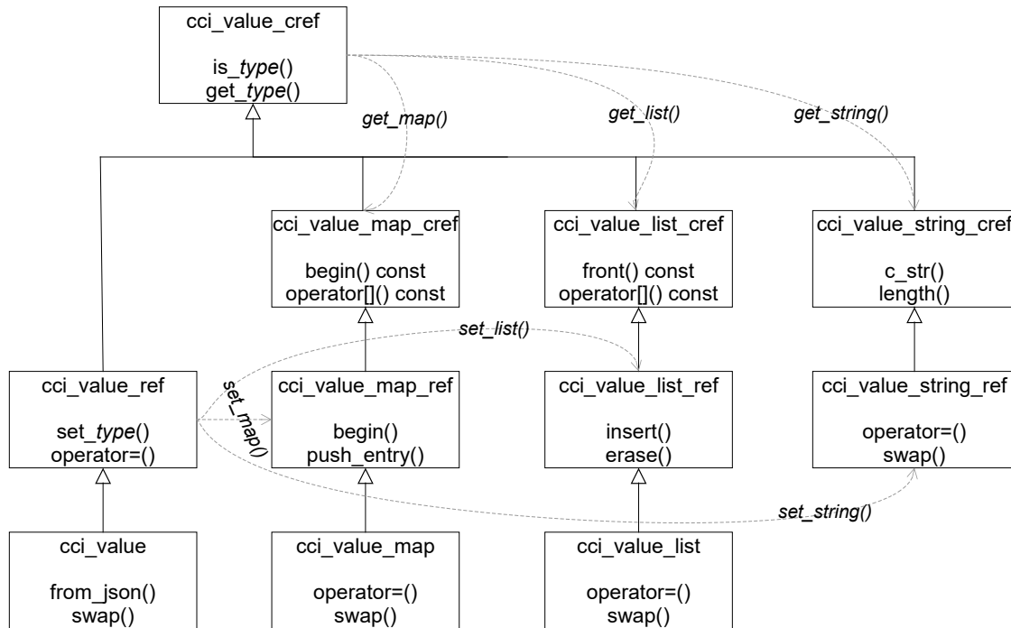
Figure 2 - cci_value hierarchy
